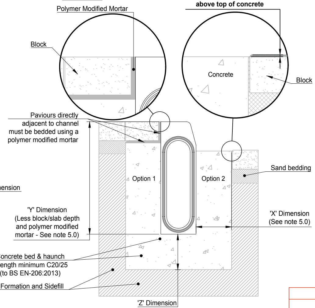
1 : 10 ACO KerbDrain KDHB Block Pavement (Option 1 and 2)
