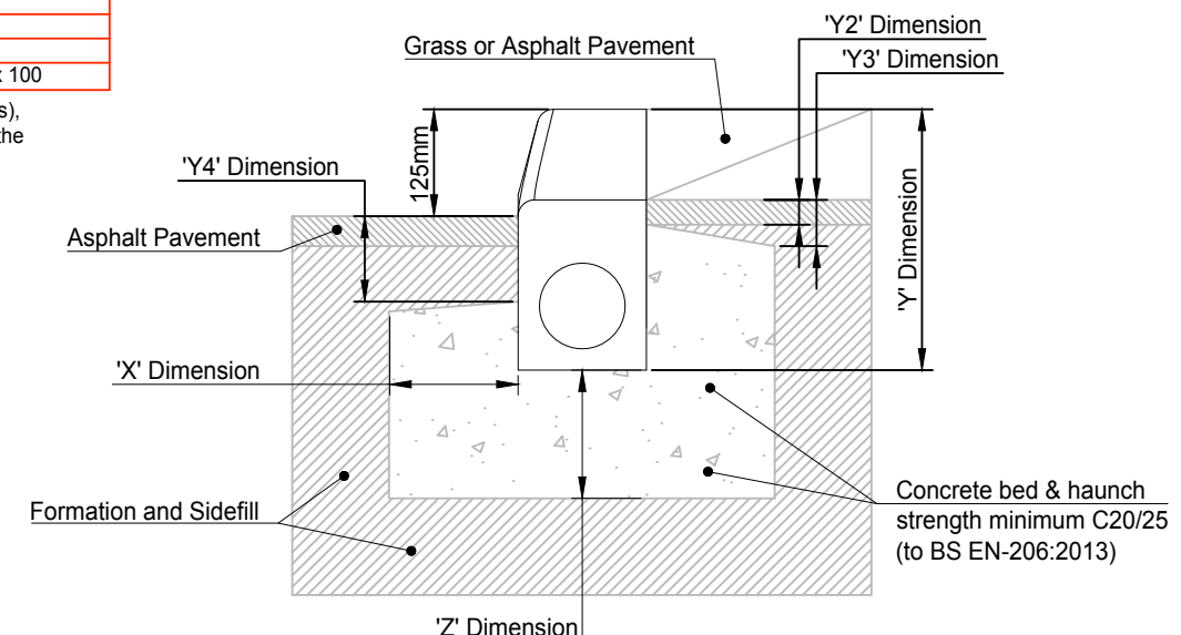
1 : 10 ACO KerbDrain KDHB Grass or Asphalt Pavement
