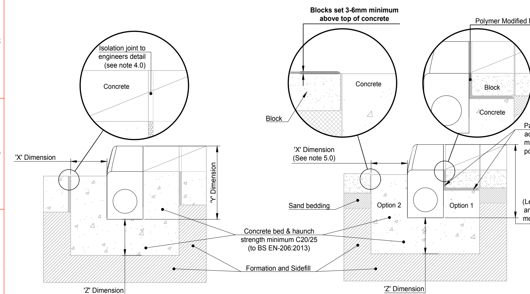
1 : 10 ACO KerbDrain KDHB Concrete Pavement
