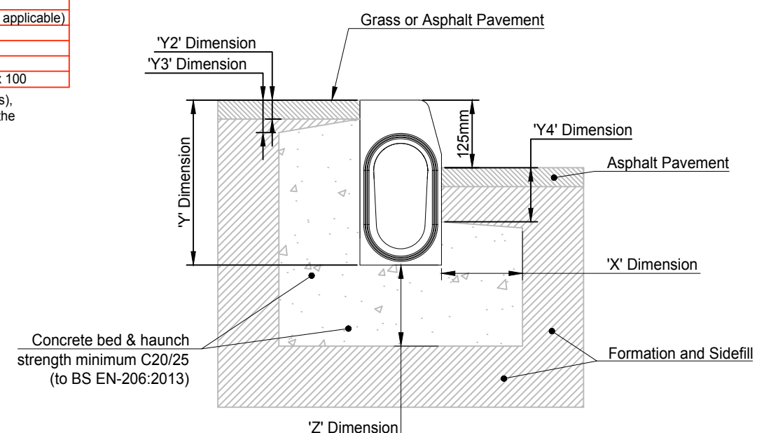
1 : 10 ACO KerbDrain KDHB Grass or Asphalt Pavement
