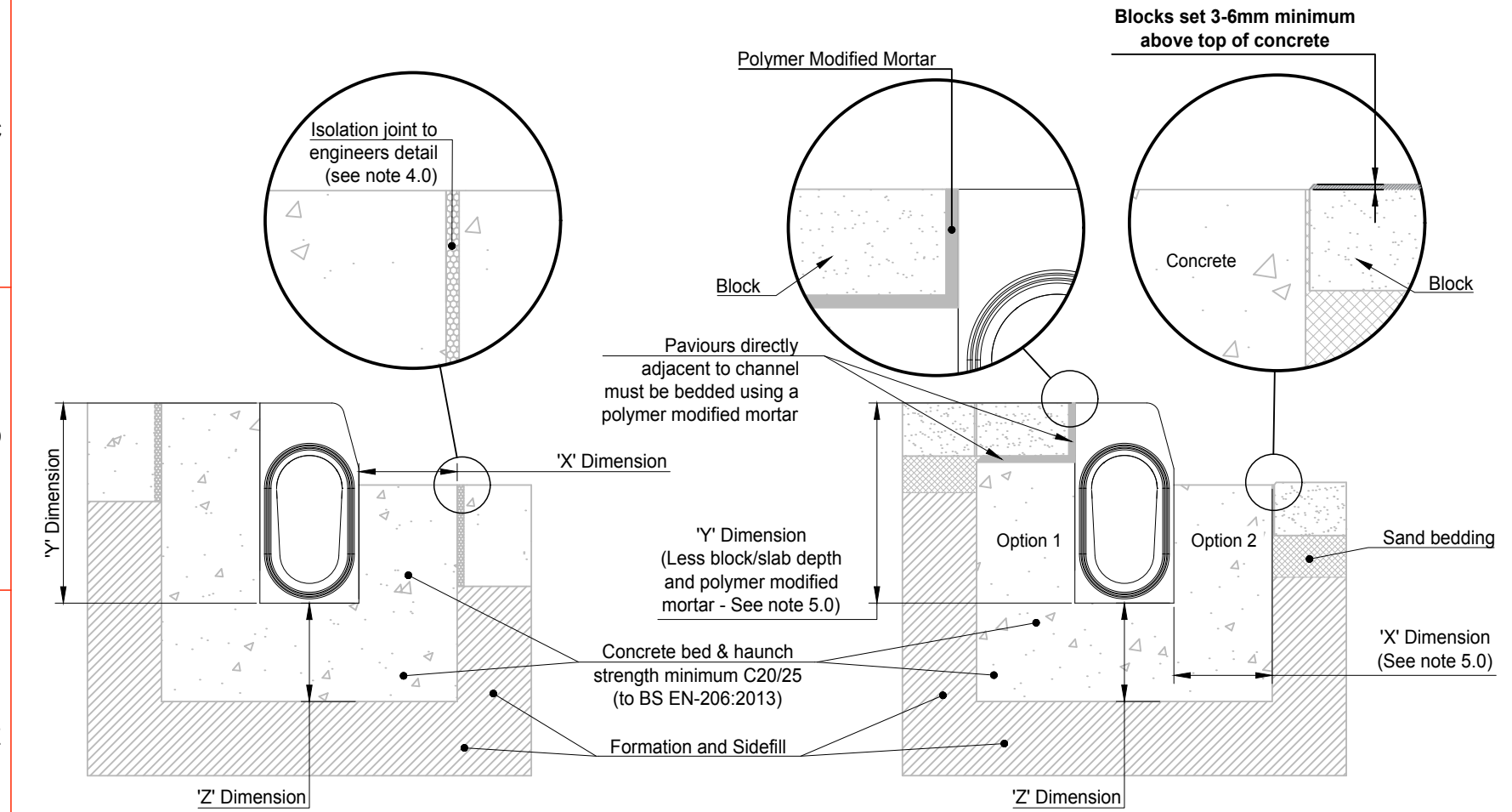
1 : 10 ACO KerbDrain KDHB Concrete Pavement
