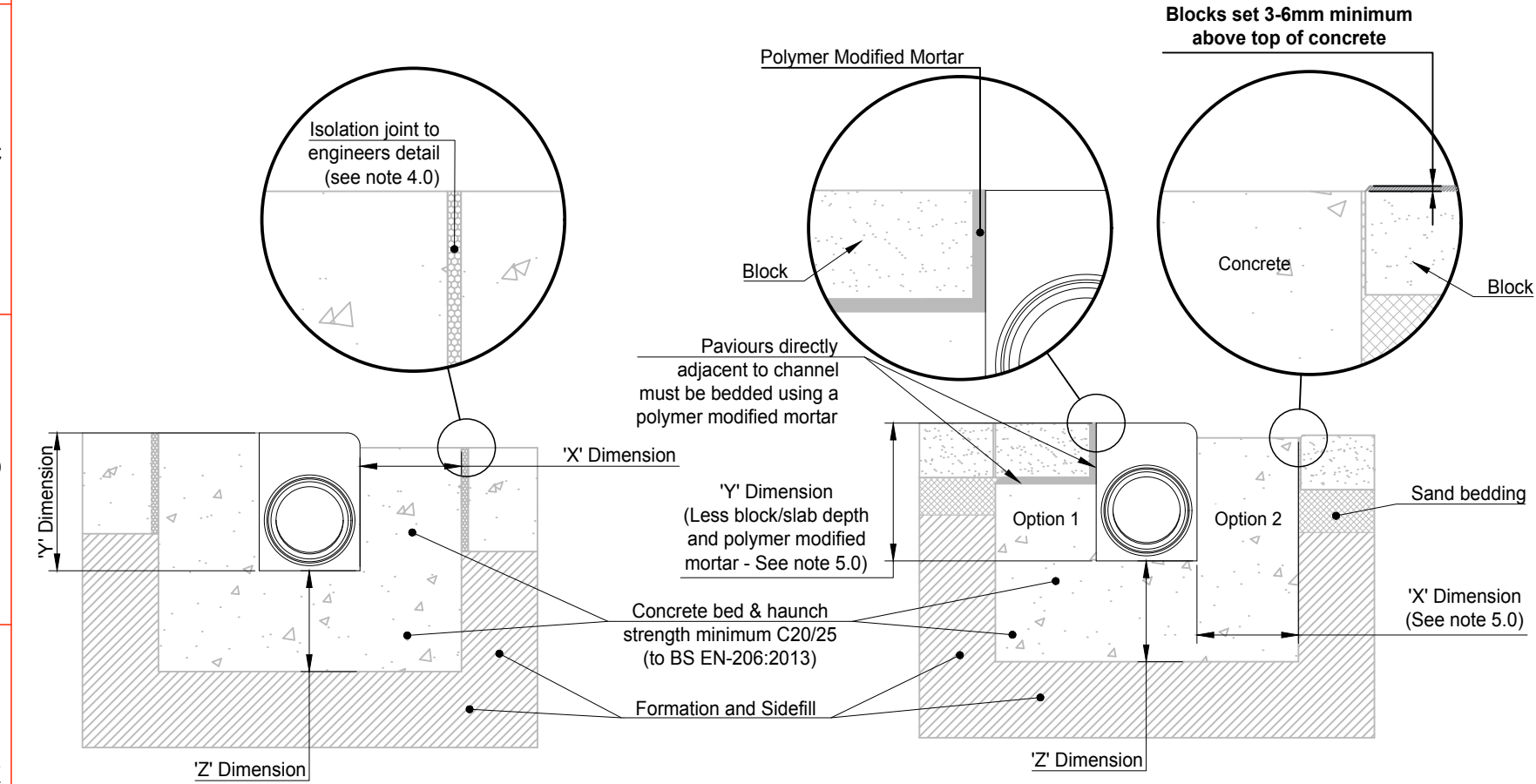
1 : 10 ACO KerbDrain KDHB Concrete Pavement
