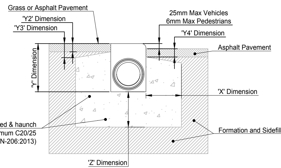
1 : 10 ACO KerbDrain KDHB Grass or Asphalt Pavement
