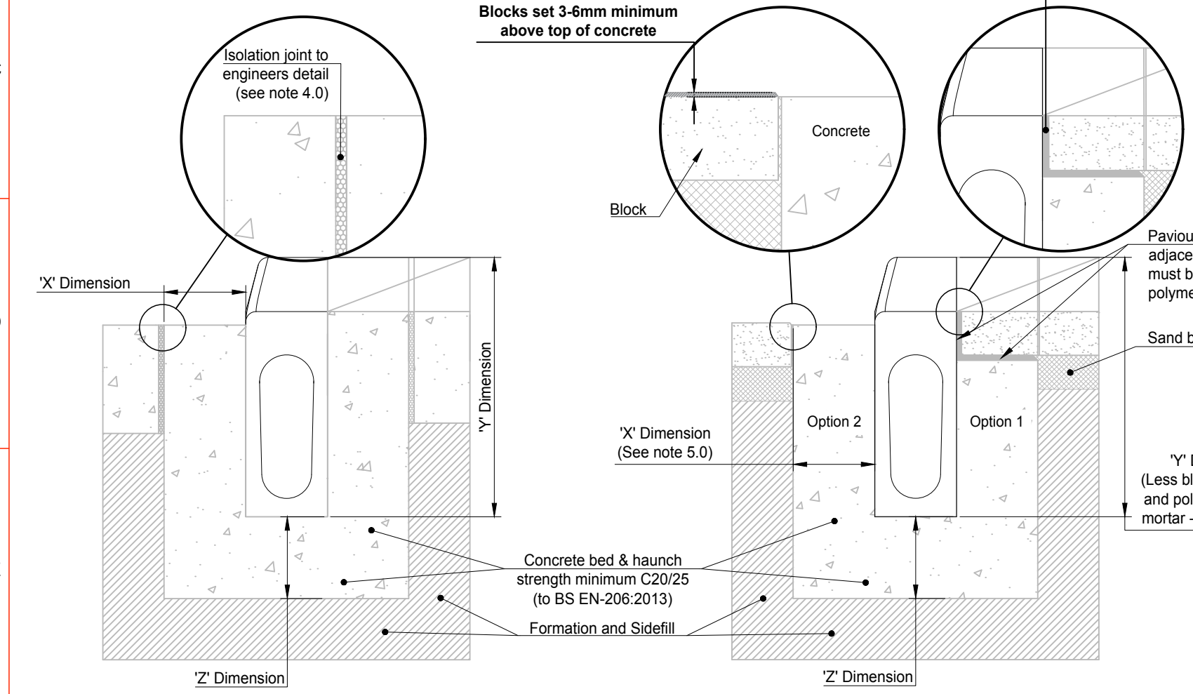
1 : 10 ACO KerbDrain KDHB Concrete Pavement
